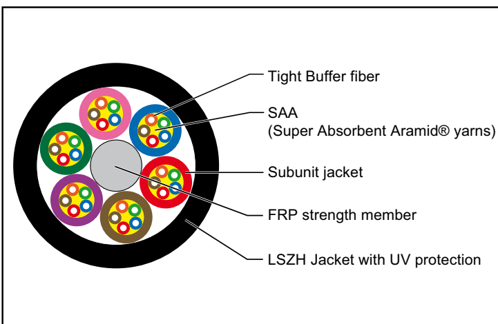
24 - 36 Fibers
