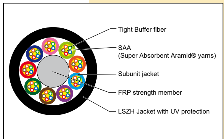
48 - 144 Fibers
