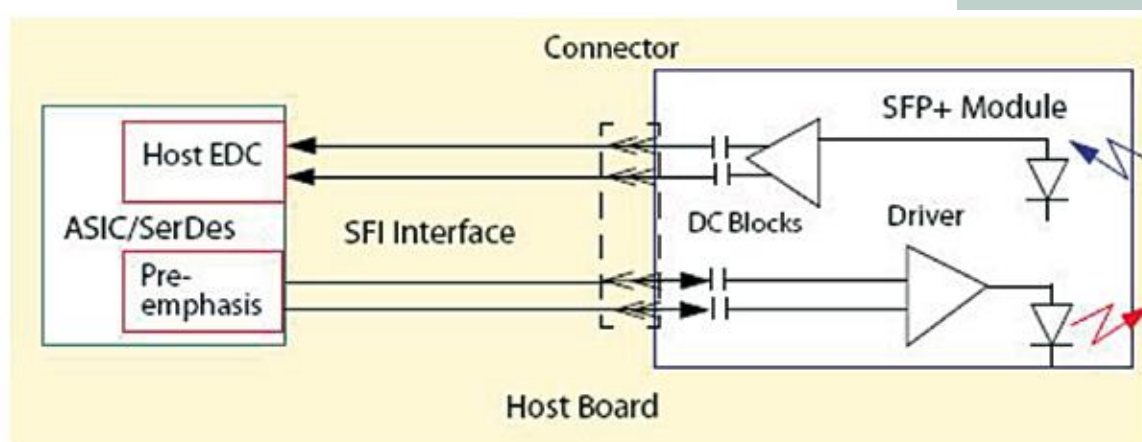
Figura 1: Interfaz al Host
