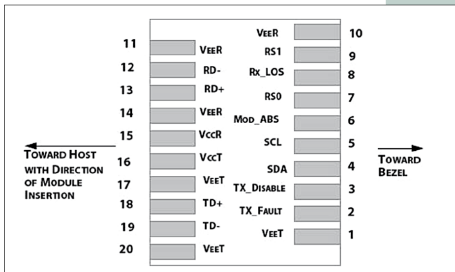
Figura 2: Interfaz al Host PCB
